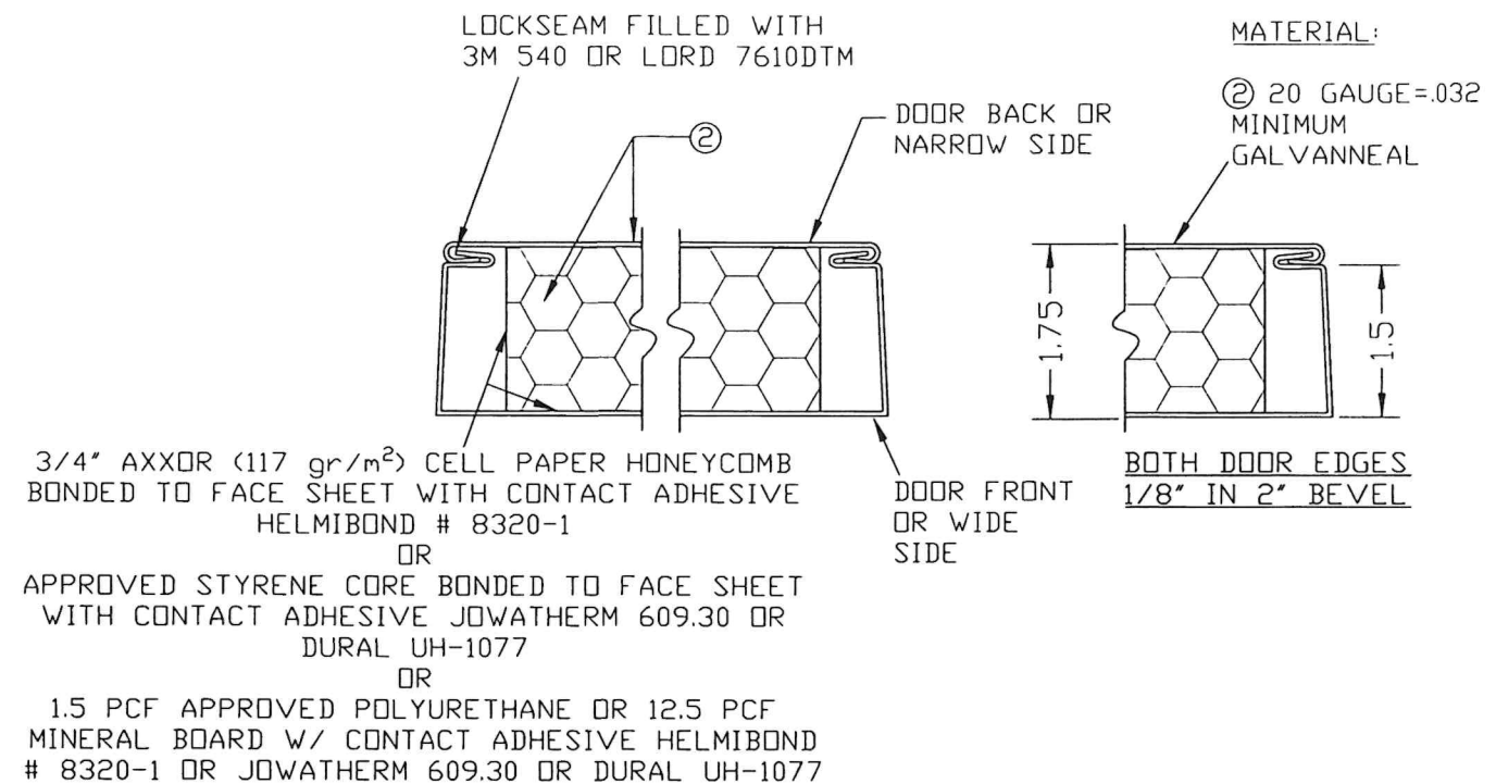
DOOR SECTION THROUGH EDGE SEAM, DETAIL X
