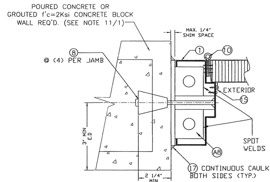
SECTION F
