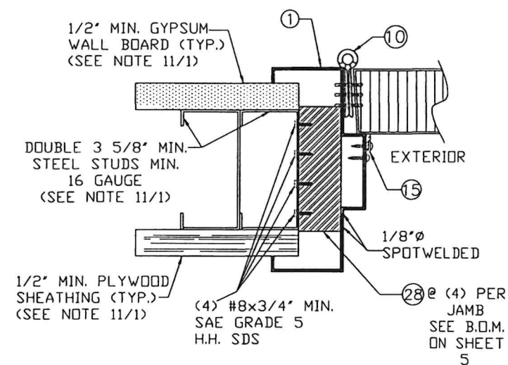
SECTION H
