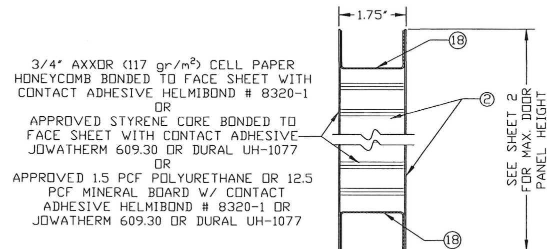
VERTICAL SECTION AT DOOR PANEL DOOR PANEL CONSTRUCTION
