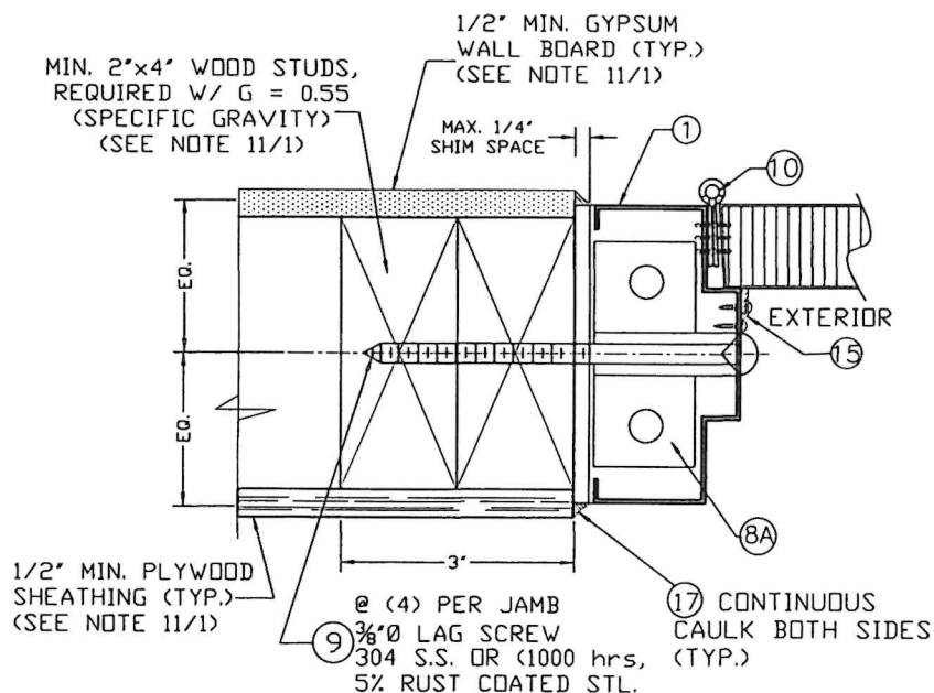
SECTION G
