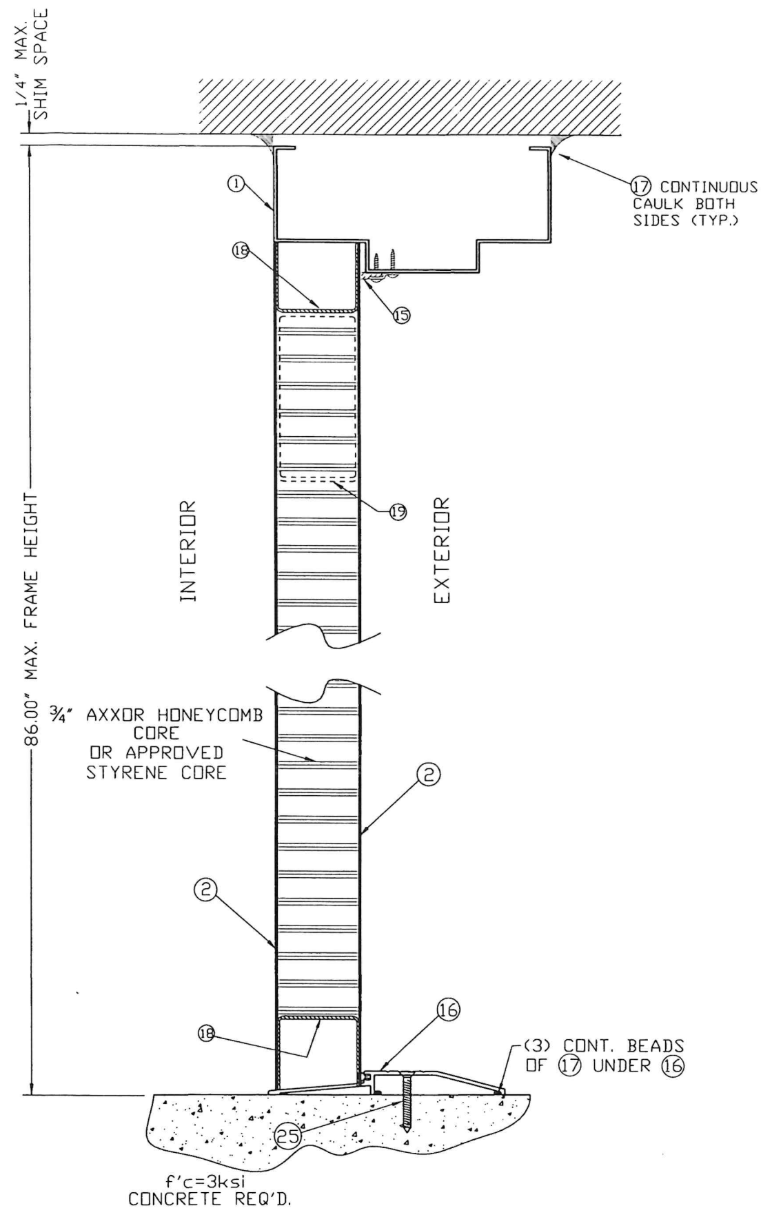
SECTIONS A1-A1 & A2-A2 AT DOOR PANEL/FRAME
