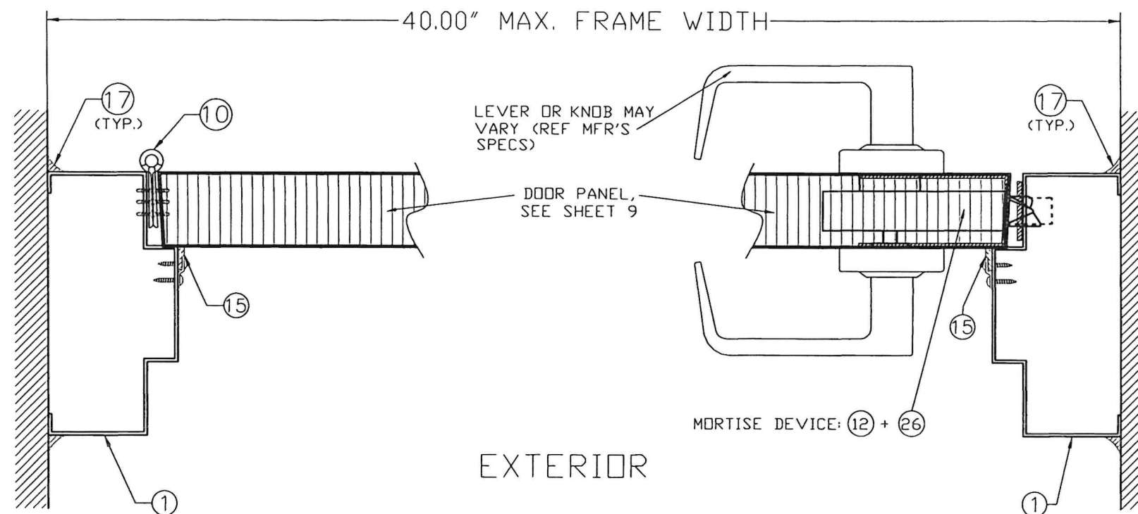
SECTION B2-B2
